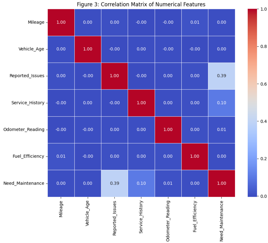
Figure 3: Correlation Matrix of Numerical Features
